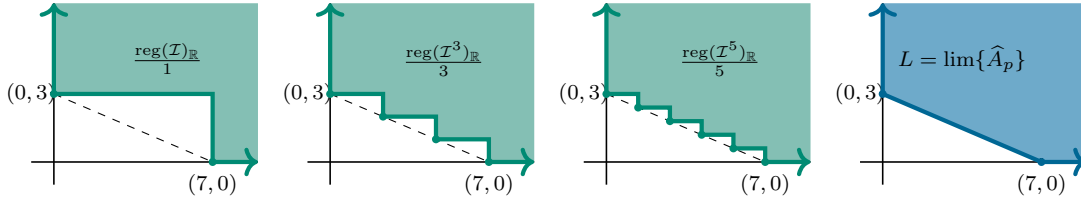
FIGURE 3. Toy picture of the convergence of \frac{\text{reg}(\mathcal{I}^p)_{\mathbb{R}}}{p} to the Seshadri region of \mathcal{I} predicted Conjecture 3.2.
